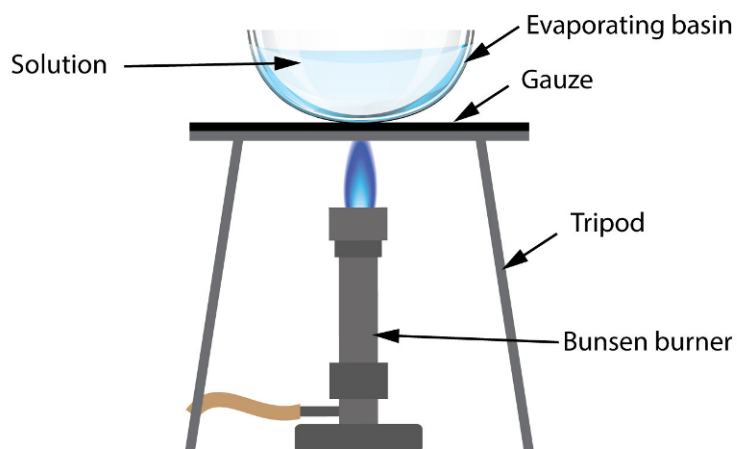
Evaporation – direct heating with a Bunsen burner
