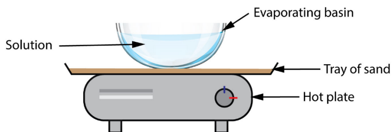
Evaporation – heating using a sand bath
