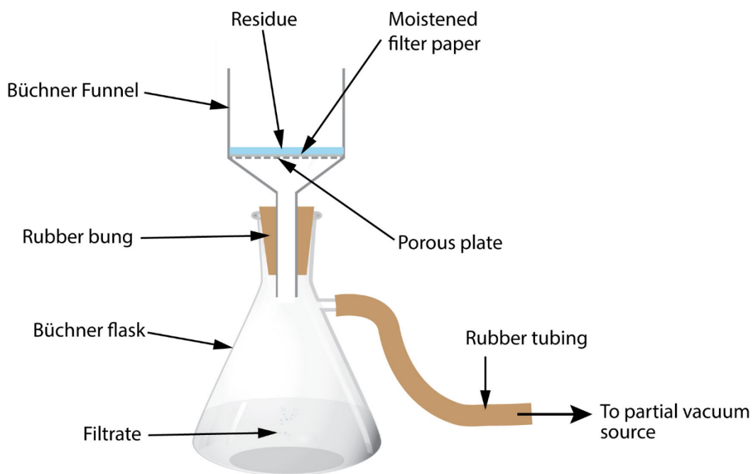
Filtration under reduced pressure
