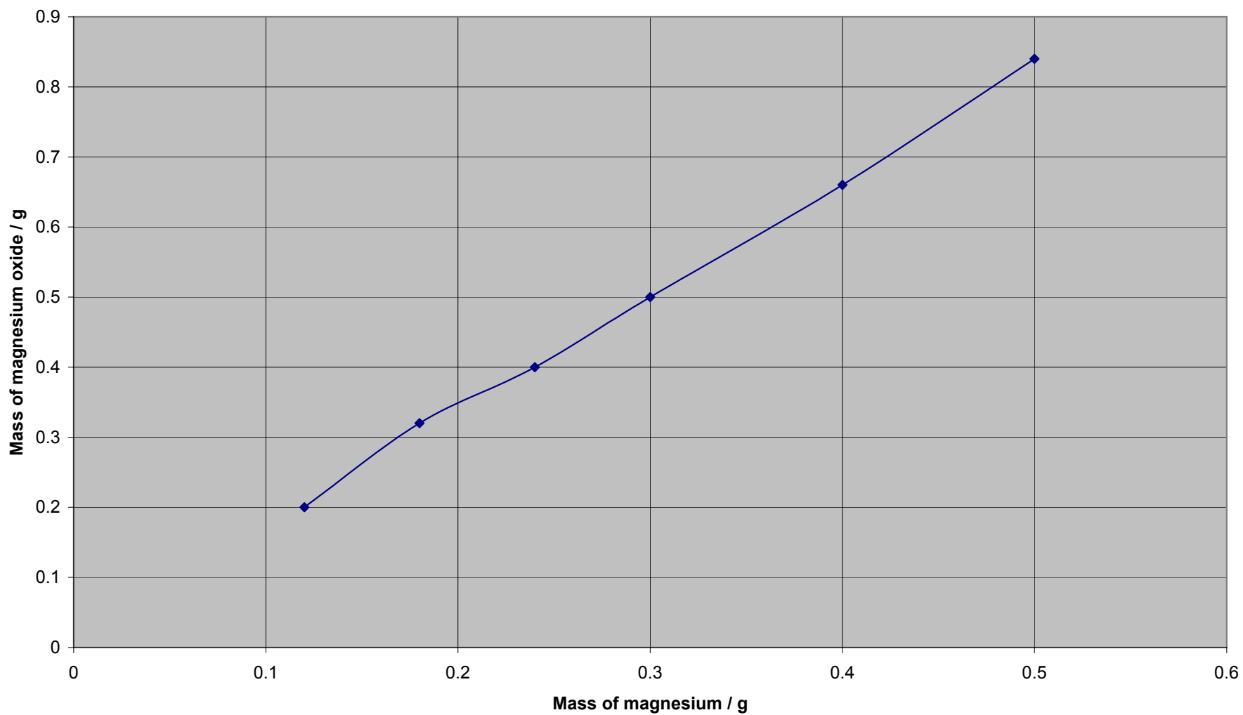
Graph of mass of magnesium against mass of magnesium oxide
