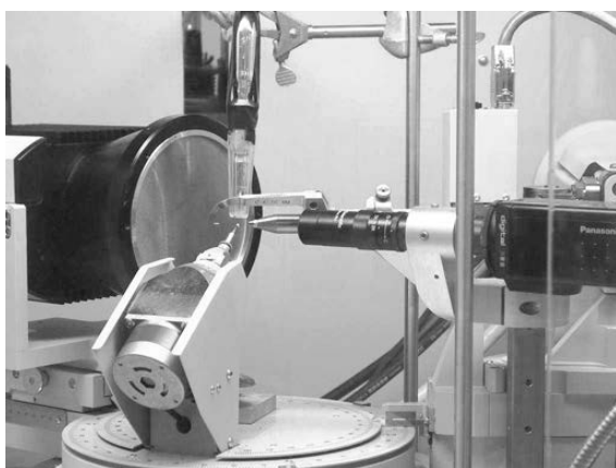
Single crystal X-ray diffractometer
