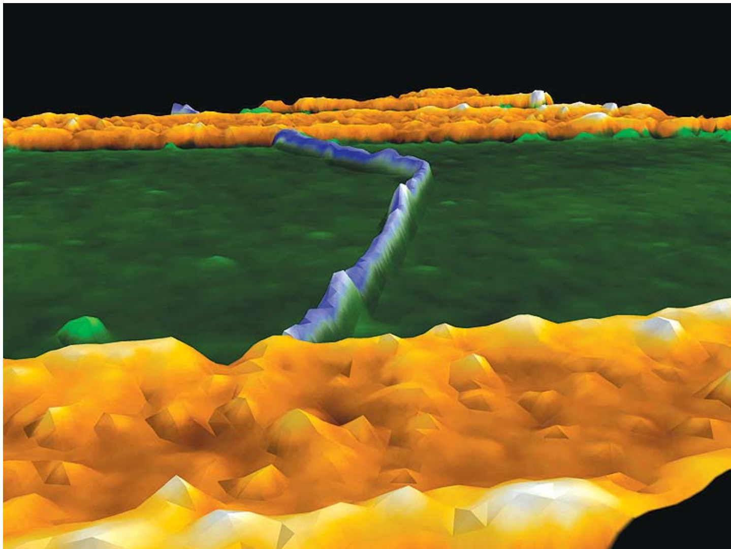
Figure 1a A 'kinked' nanotube joining electrodes (yellow) on a silicon dioxide base (green)
