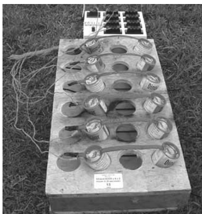
Electrical firing systems for fireworks displays
