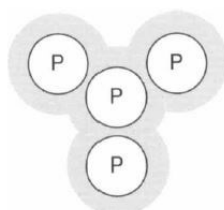
Figure 7.12 A representation of the tetrahedral phosphorus molecule
