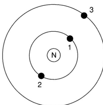
Figure 7.2 A simple representation of an atom
