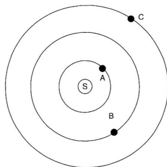
Figure 7.3 A simple representation of a solar system
