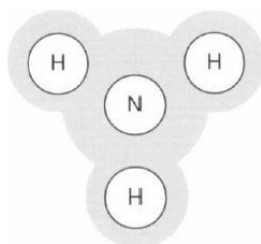
Figure 7.11 A representation of the pyramidal ammonia molecule
