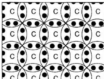
Figure 7.14 Part of the giant covalent structure of carbon
