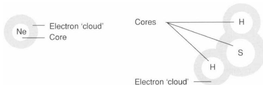
Figure 7.9 Representing molecules with electron clouds
