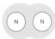
Figure 7.10 A representation of a nitrogen molecule
