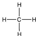
Figure 7.5 A representation of a methane molecule
