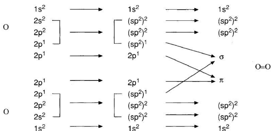
Figure 7.4 A scheme to show the orbitals in a simple molecule
