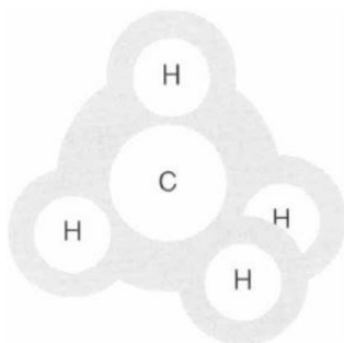
Figure 7.8 A fourth representation of a methane molecule
