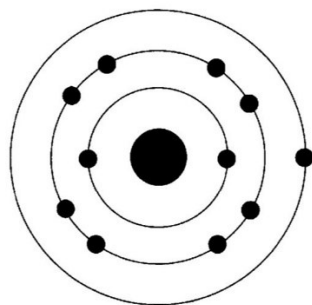
Figure 7.1 A typical representation of an atom
