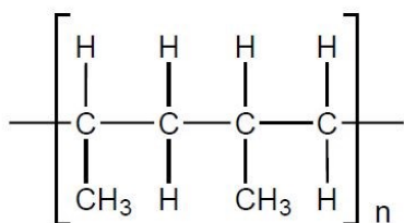
Polypropene
