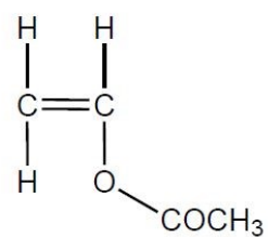
Vinyl acetate
