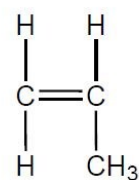
Propene
