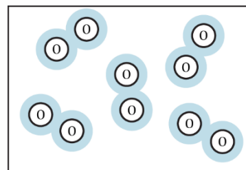
9. Oxygen gas
