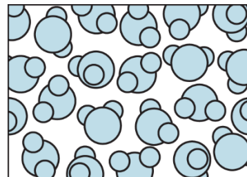
6. Liquid water
