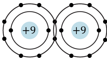
7. Fluorine molecule
