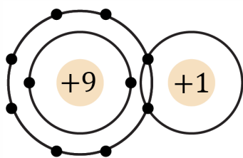
4. Hydrogen fluoride molecule
