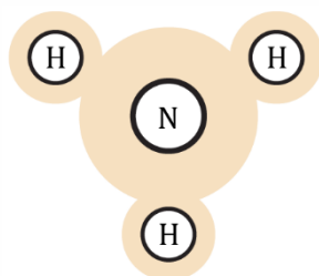
8. Ammonia molecule
