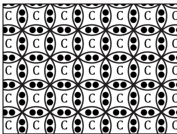
2. Diamond lattice
