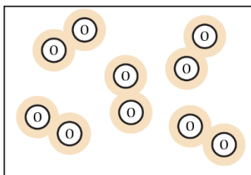
5. Oxygen gas
