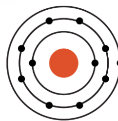
6. Sodium atom
